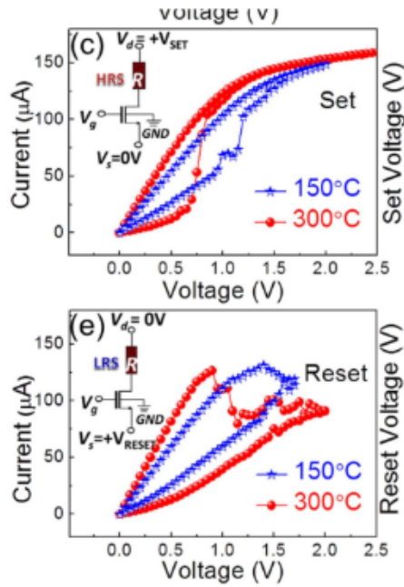
Fig. 8. Measured I - V characteristics of the integrated 1T1R \text{HfO}_2 cell from [4], comparing two atomic layer deposition temperatures (150 °C in blue and 300 °C in red). Top: SET; Bottom: RESET. The 300 °C deposition produces tighter resistance distributions and lower switching voltages. Reproduced from [4].
