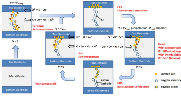
Fig. 4. Operation of a VCM cell. Starting from the as-fabricated insulating state, a forming pulse nucleates a conductive filament of oxygen vacancies. Subsequent SET pulses reconnect the filament to enter the LRS; RESET pulses partially rupture the filament to return to the HRS. Reproduced from [1].
