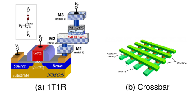
Fig. 6. Competing RRAM array architectures. (a) 1T1R: a CMOS NMOS in the front-end with the \text{HfO}_2/\text{Ti}/\text{TiN} MIM stack between metals 2 and 3. Reproduced from [4]. (b) Passive crossbar with bitlines, wordlines, and resistive memory at every intersection. Reproduced from [3].
